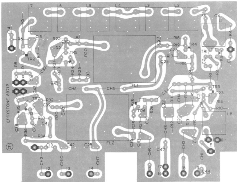
SELECTIVITY MODULE
